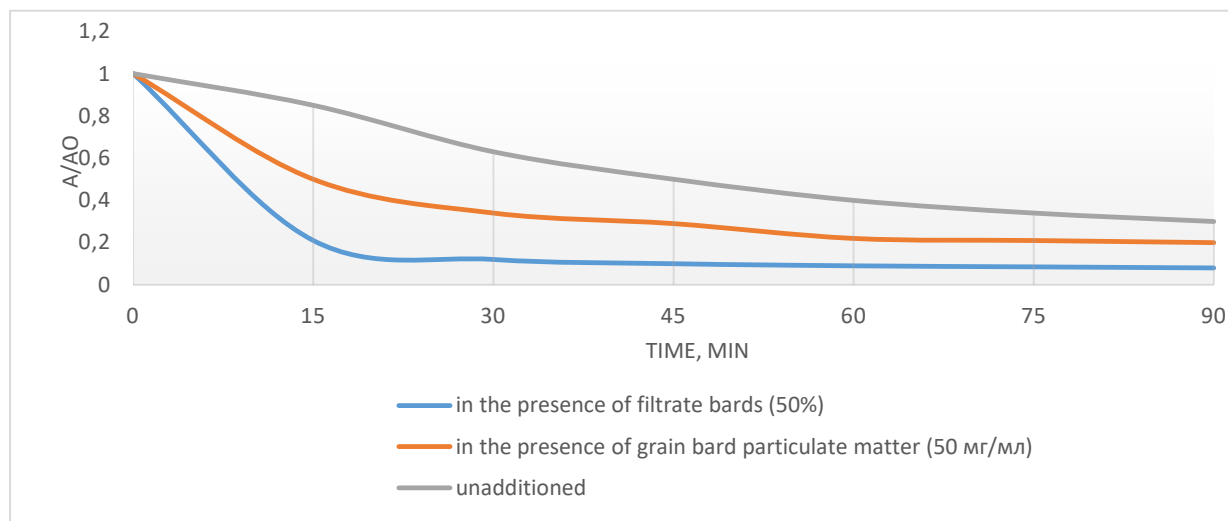
Fig. 3. Stability of neutral proteins under different conditions
