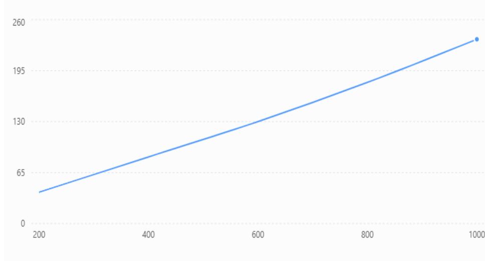
Figure 2. Dependence of the total power output of the hybrid photovoltaic-thermoelectric (PV-TEG) system on solar irradiance.
