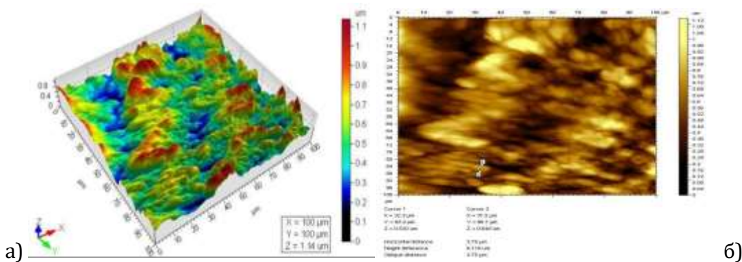
Figure 1. AFM images of a composite material based on polyethylene with nitrogen-, phosphorus-, metal-containing oligomers a) - three-dimensional image, b) - two-dimensional image.
