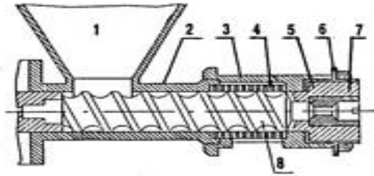
Figure 1. A simplified screw press. 1-funnel body .2-body. 3- press 4- perforated cylinder . 5- sleeve (bubble). 6- lock-nut . 7-filter. 8-screw
